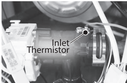
Figure 66 - Water inlet thermistor location
