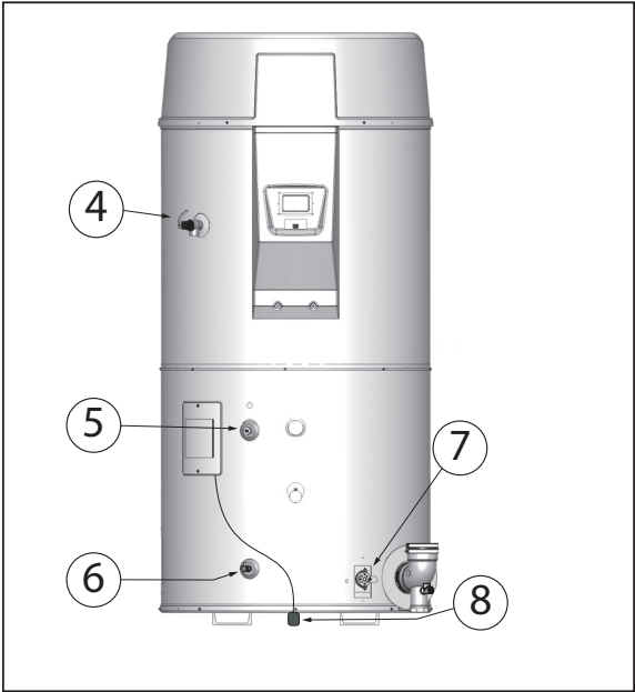
Figure 5. Locating the T&P Valve, Lower Temperature Probe, and Drain Valve
