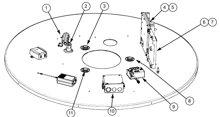
Figure 9. Inner Cover Control Assembly
