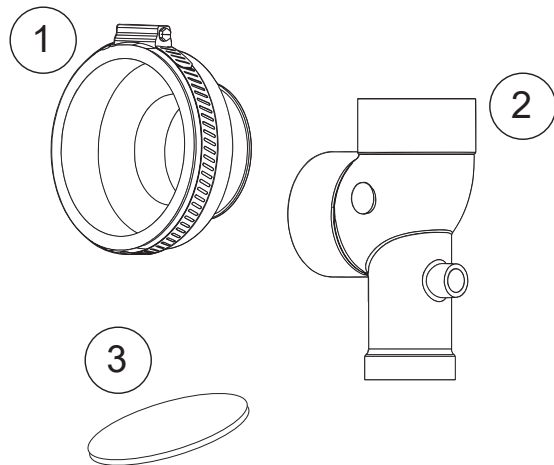
Figure 12. 3" Exhaust Connector Kit
