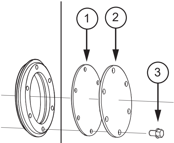
Figure 4. Cleanout Assembly
