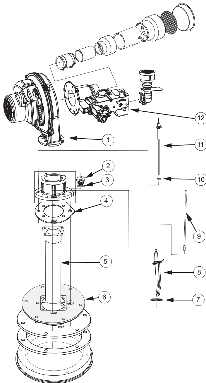
Figure 10. 220-Gallon Blower-Burner Assembly
