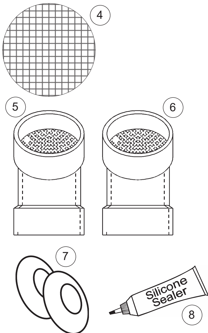
Figure 13. 3" Vent Kit
