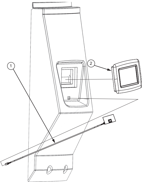
Figure 6. Display Assembly
