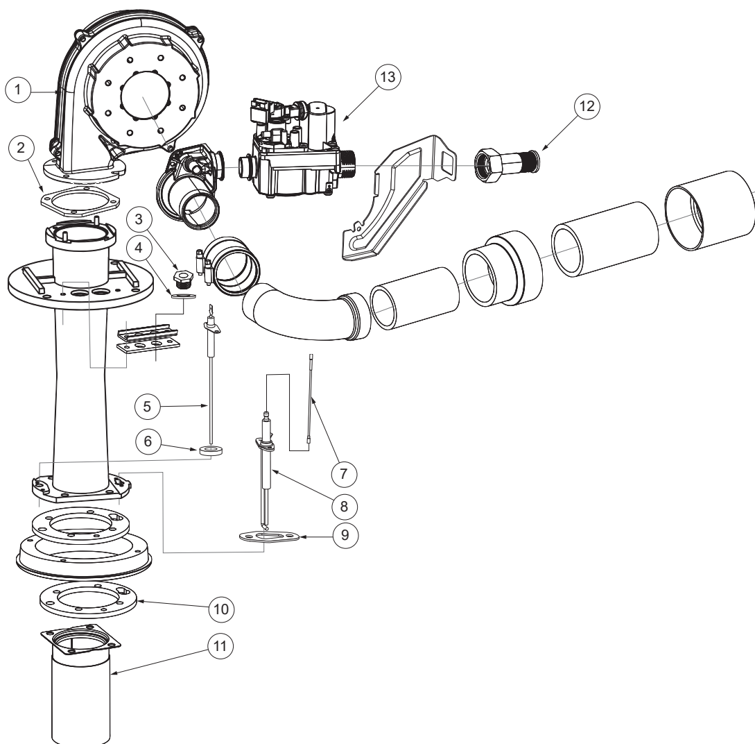
Figure 7. Blower/Burner Assembly
