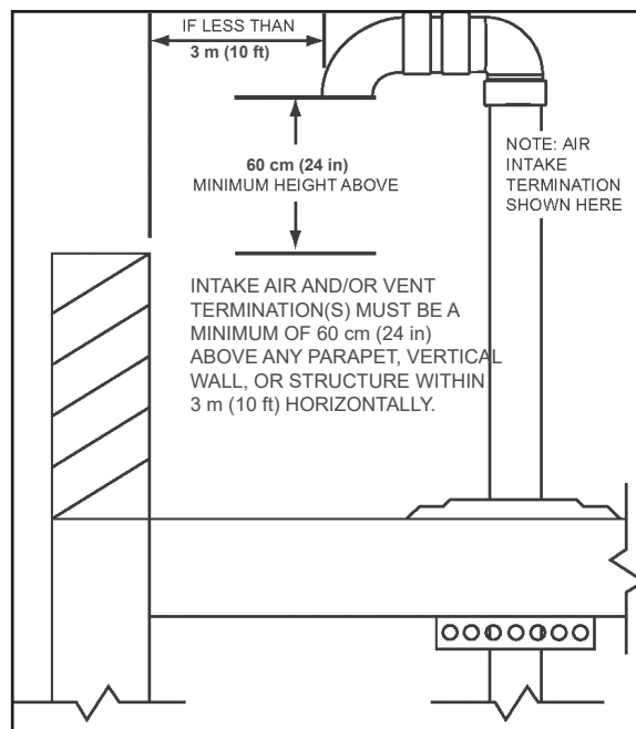
Figure 22. Vertical Terminations Parapet Clearances
