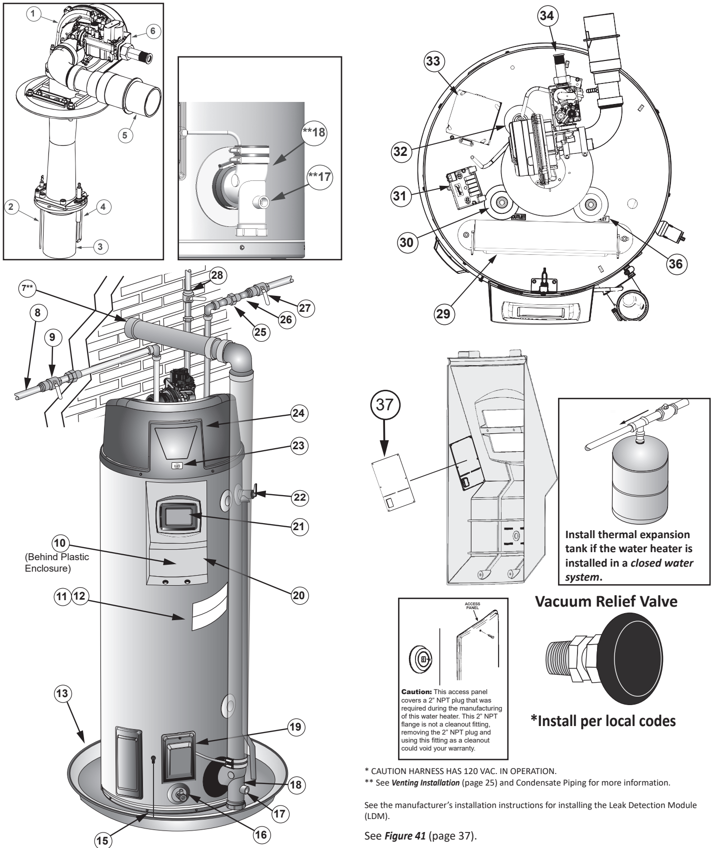
Figure 1. 50-Gallon Unit
