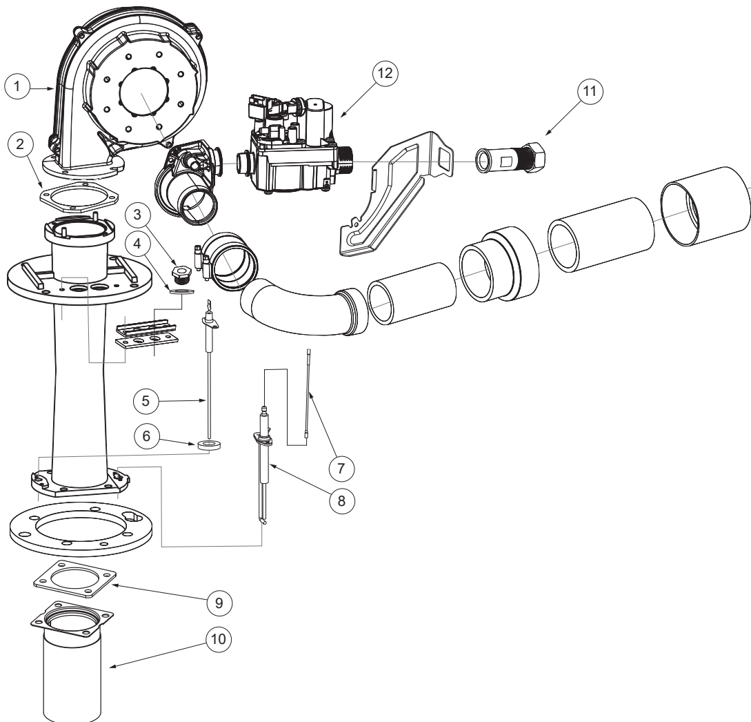
Figure 7. Blower/Burner Assembly
